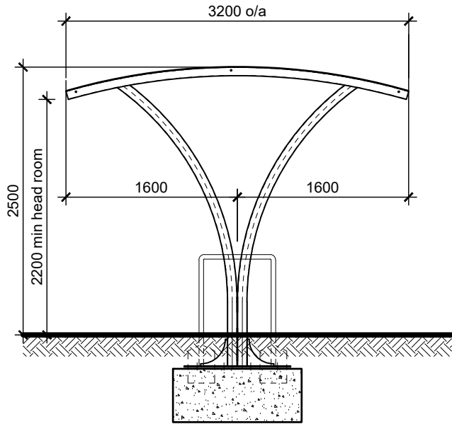
Shelter Secondary Elevation
