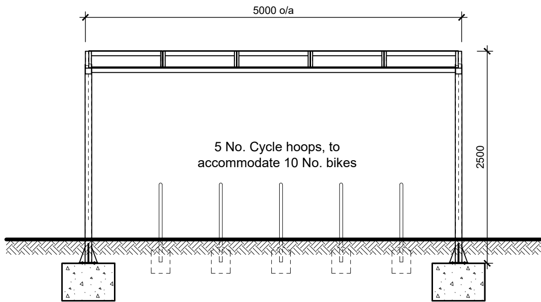
Shelter Primary Elevation
