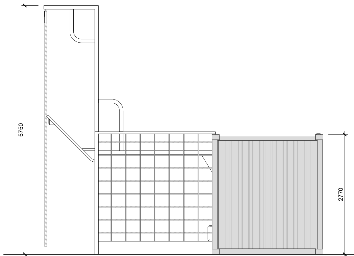
ELEVATION 03
