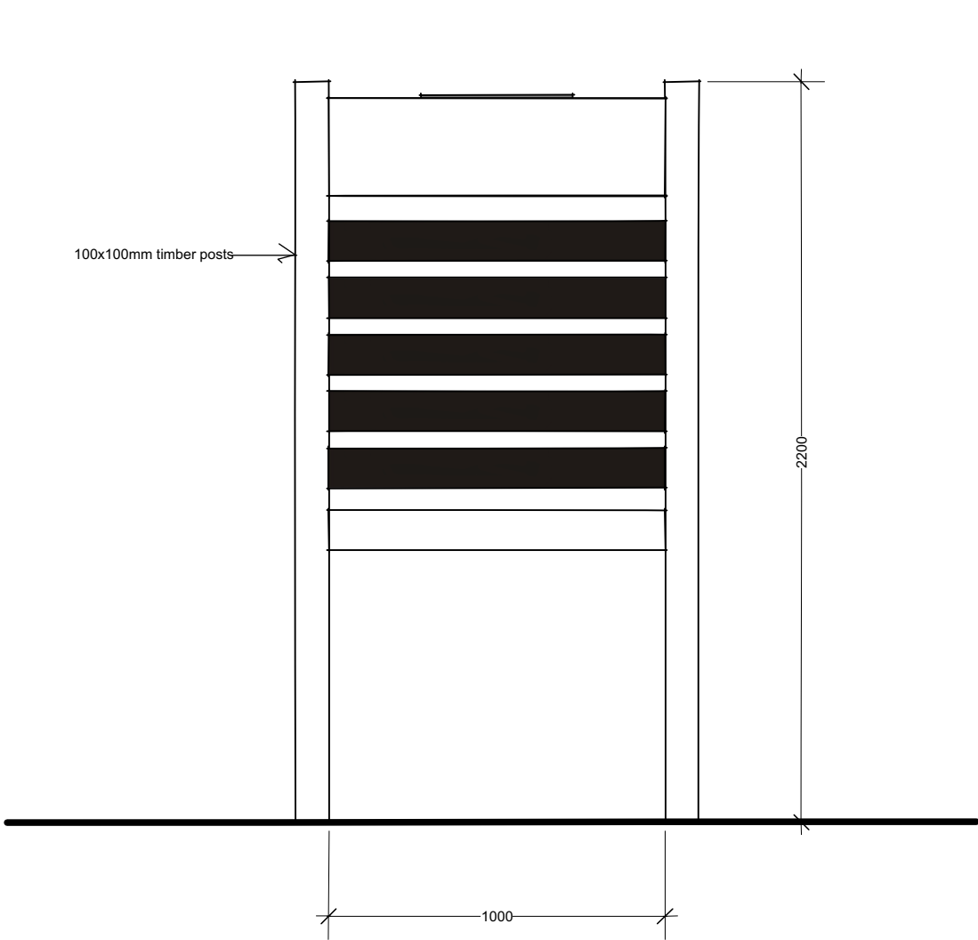
Rear Elevation
