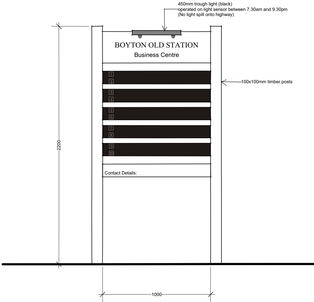
Front (Road Facing) Elevation
