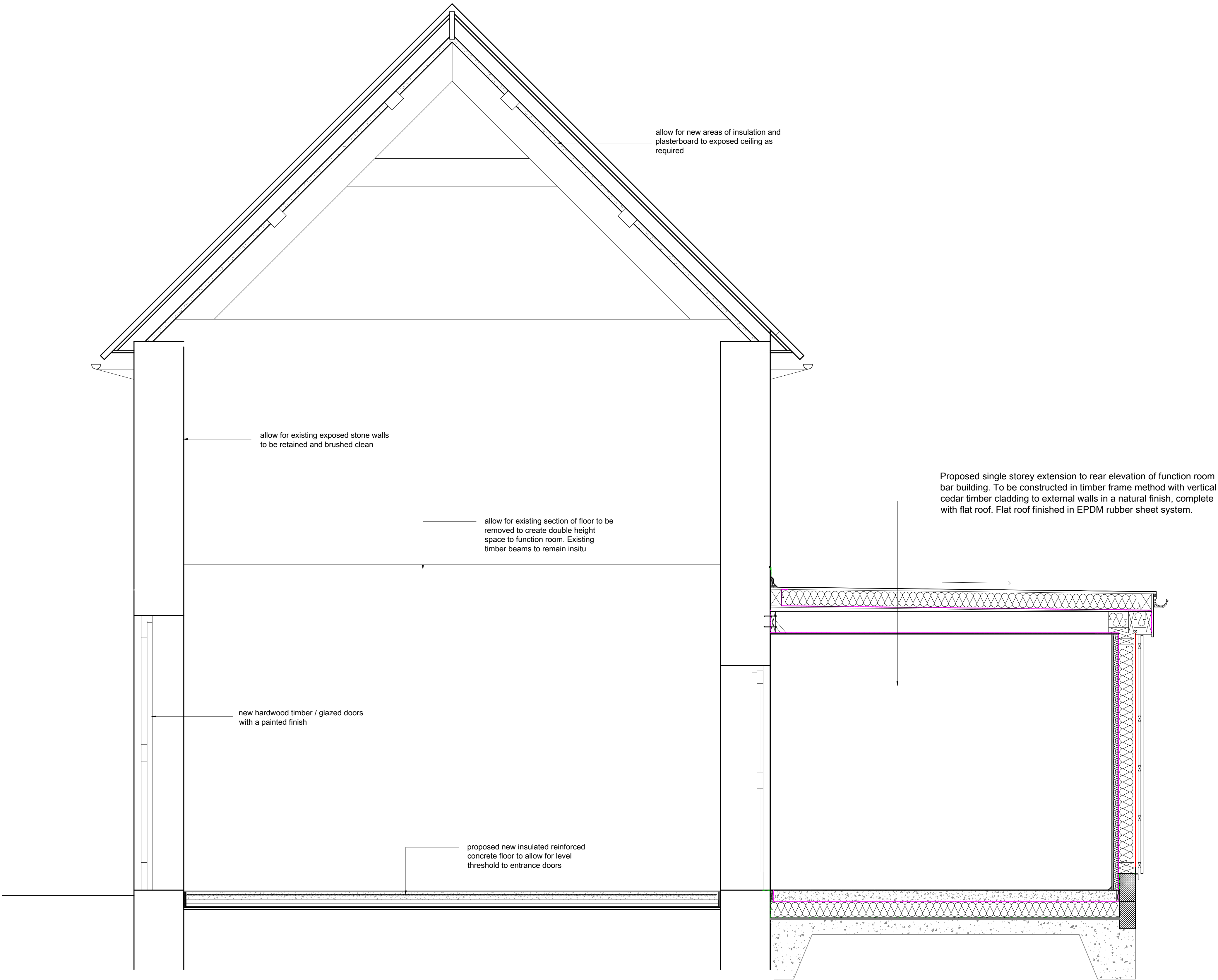
Proposed section A~A Scale 1:20 @ A1
