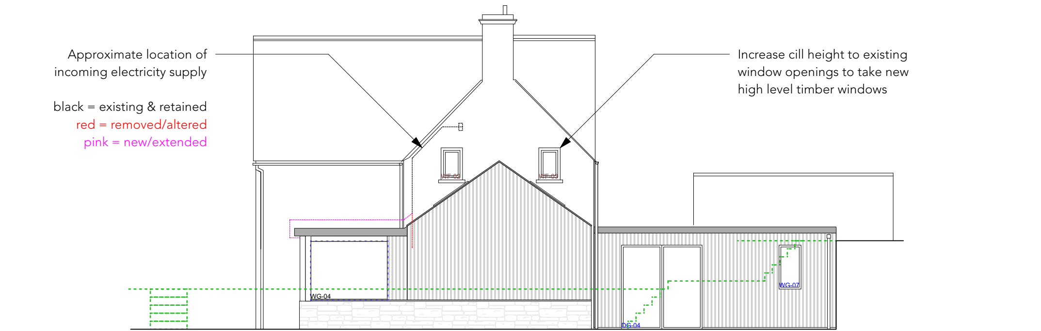
North-West elevation
