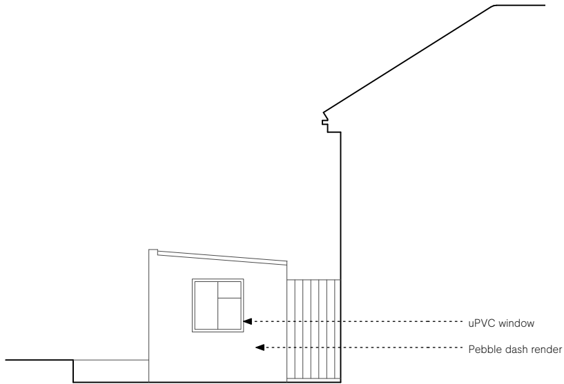
Front elevation
