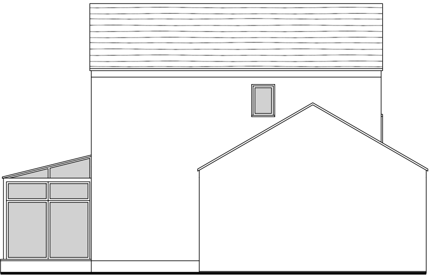
SOUTH-EAST ELEVATION
