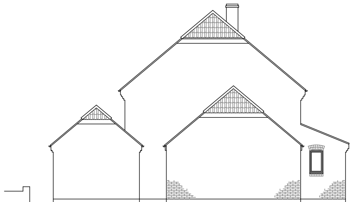
EXISTING END ( EAST ) ELEVATION 1:100
