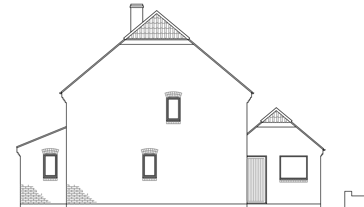
EXISTING SIDE ( WEST ) ELEVATION 1:100
