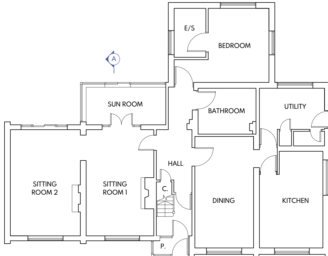
GROUND FLOOR 1:100
