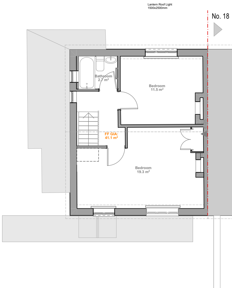
1. 1. Existing First Floor Plan 1:100
