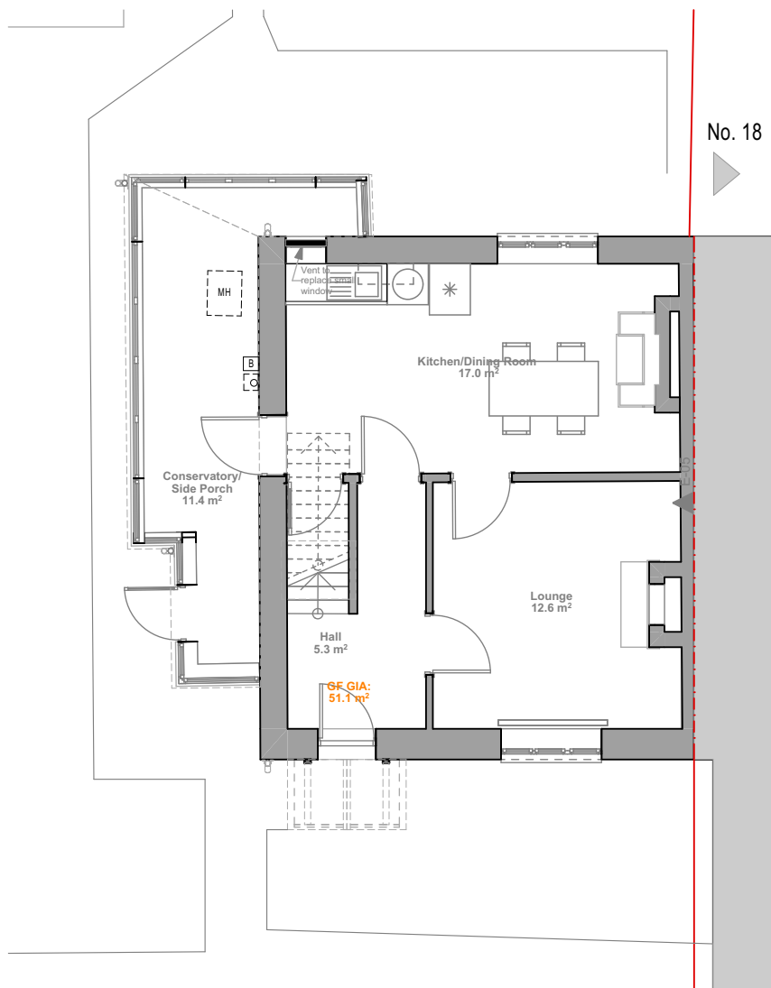
0. 0. Existing Ground Floor Plan 1:100
