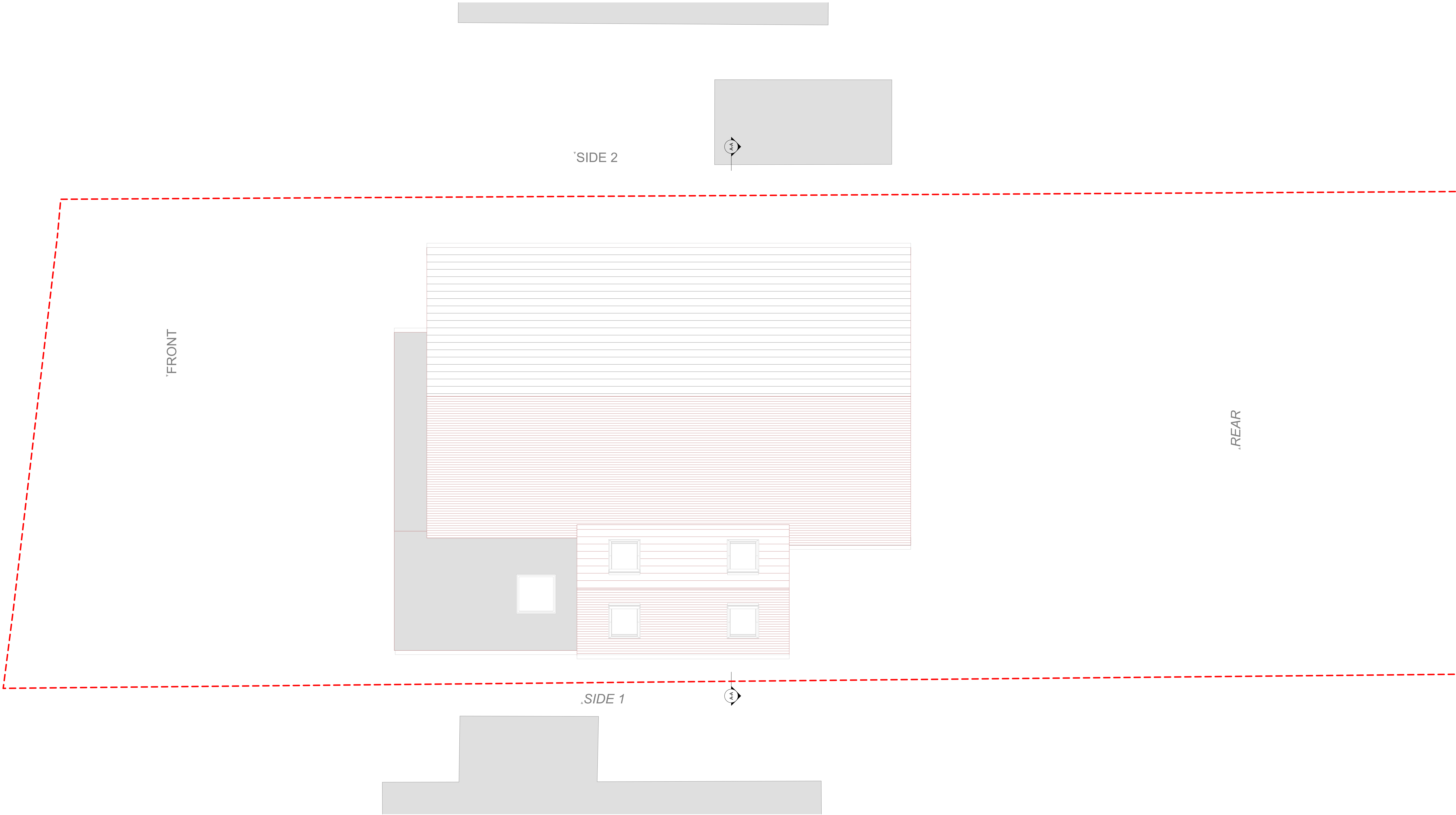
+02-Eaves/Loft Floor - Proposed
