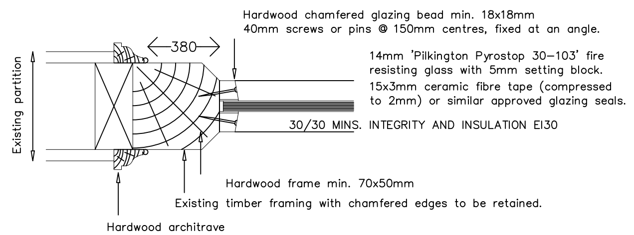
Horizontal Section
