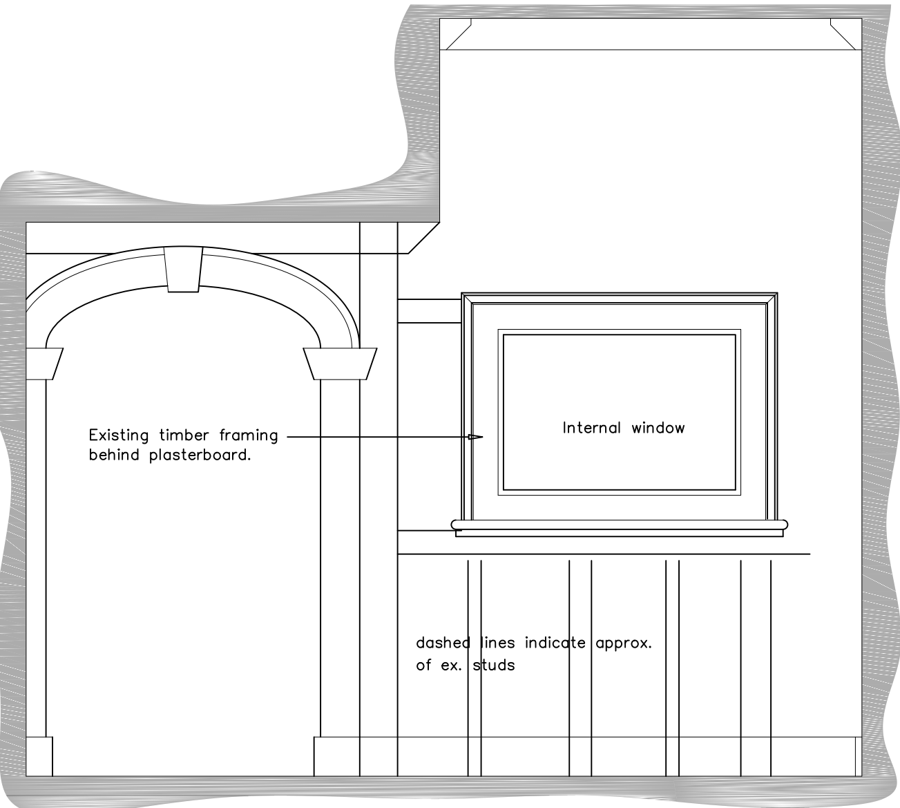
Room Elevation From Entrance Stairwell G04 1:20
