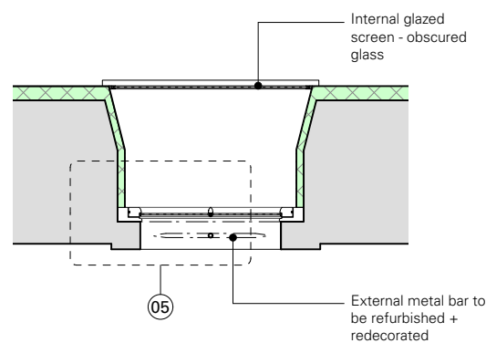
04 Plan as proposed- 1:25
