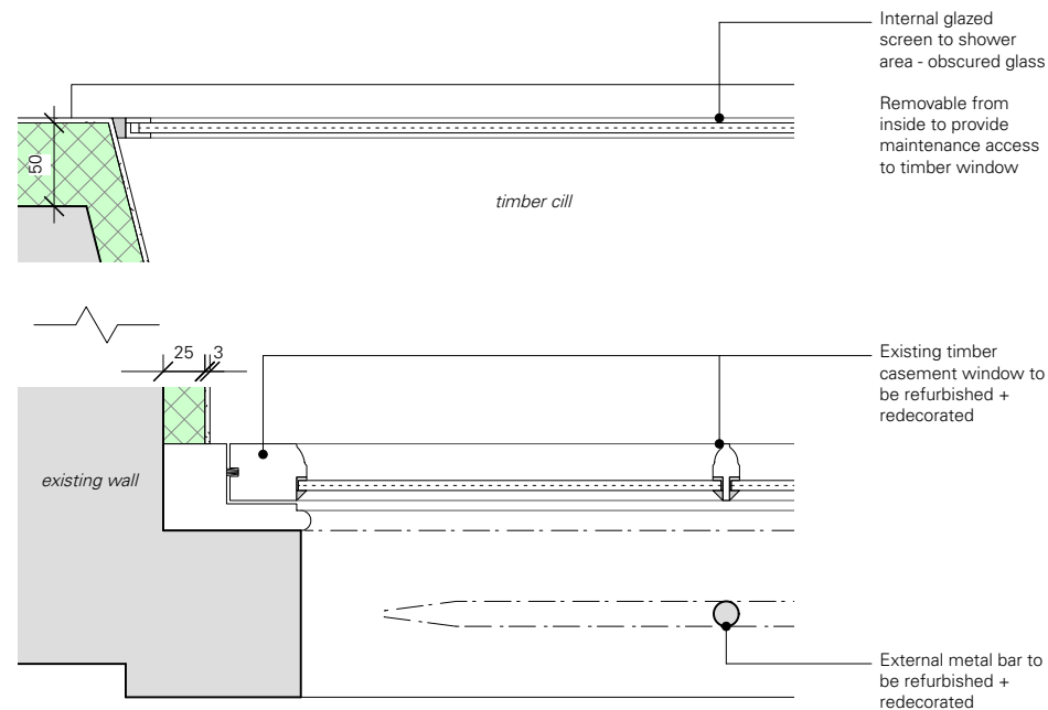
05 Plan detail - 1:5
