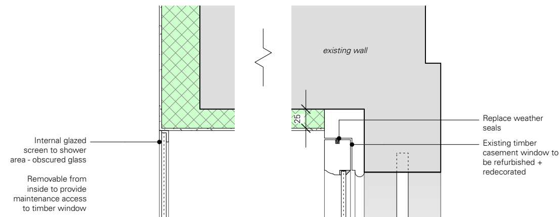
03 Section detail - 1:5
