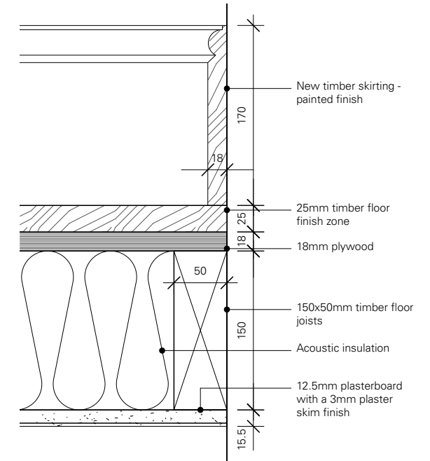
07 Proposed floor build-up - 1:5
