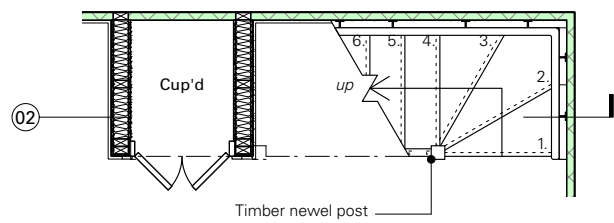
04 Ground floor plan as proposed - 1:50
