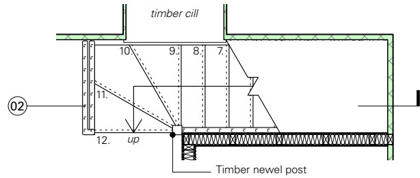
03 First floor plan as proposed - 1:50
