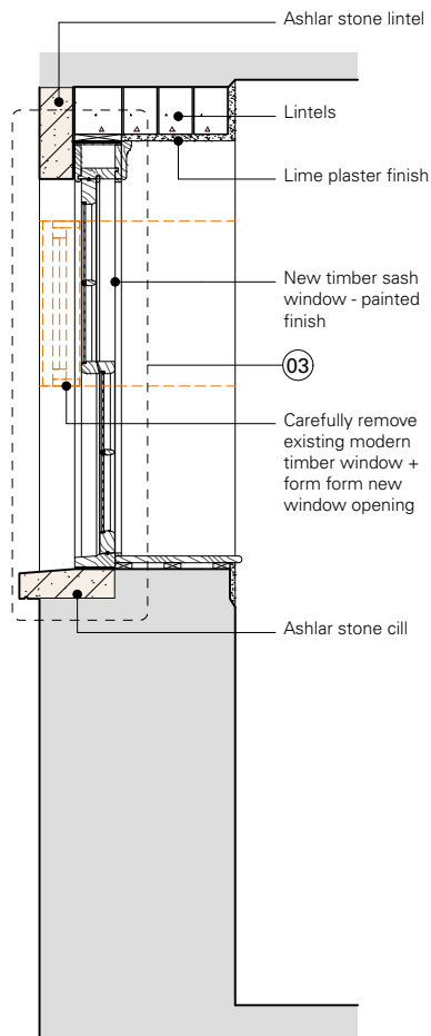
02 Section as proposed - 1:25
