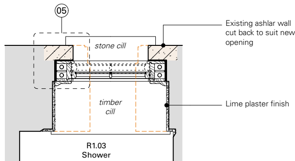
04 Plan as proposed- 1:25
