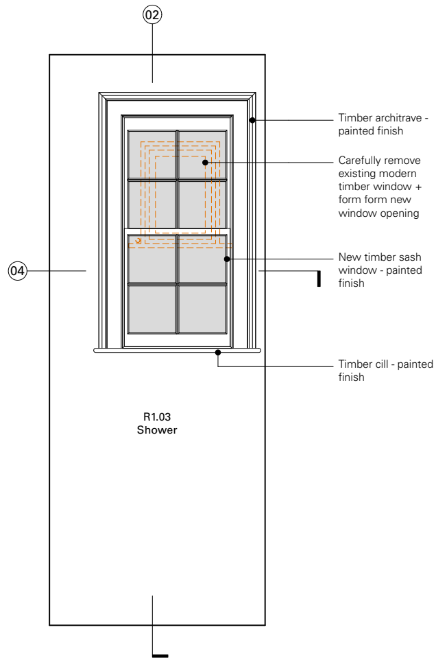
01 Elevation as proposed - 1:25
