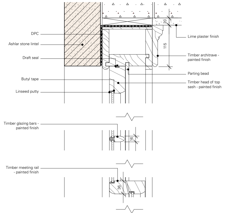
03 Section detail - 1:5
