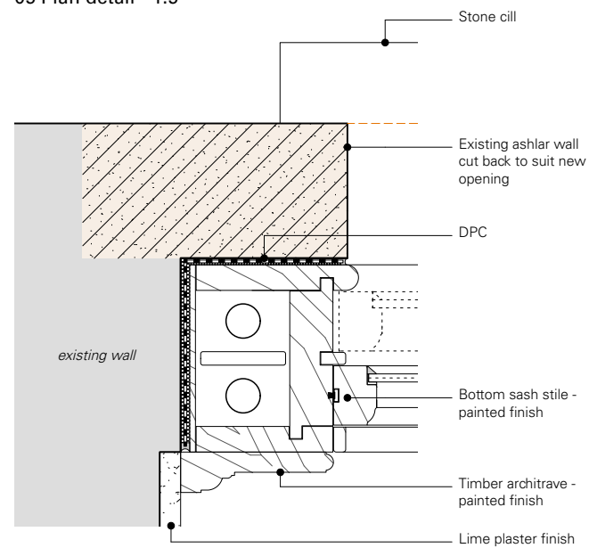
05 Plan detail - 1:5
