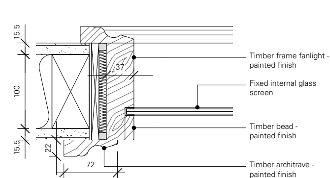
08 Fixed screen plan detail - 1:5
