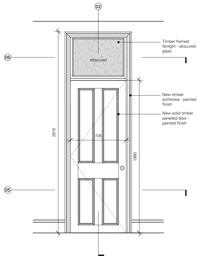
01 Elevation as proposed - 1:25
