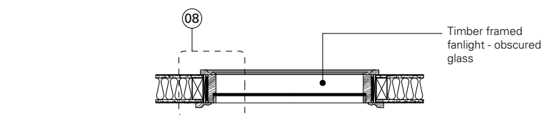
06 Fixed screen plan - 1:25
