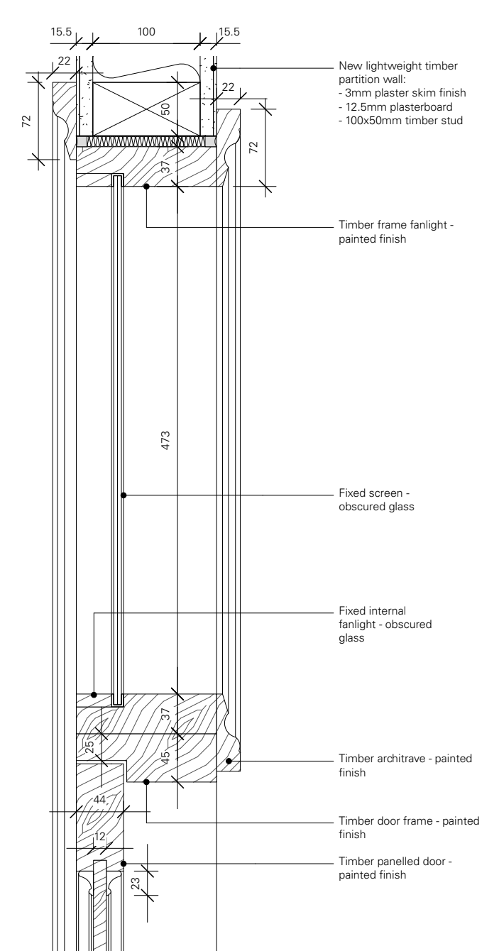
04 Head detail - 1:5
