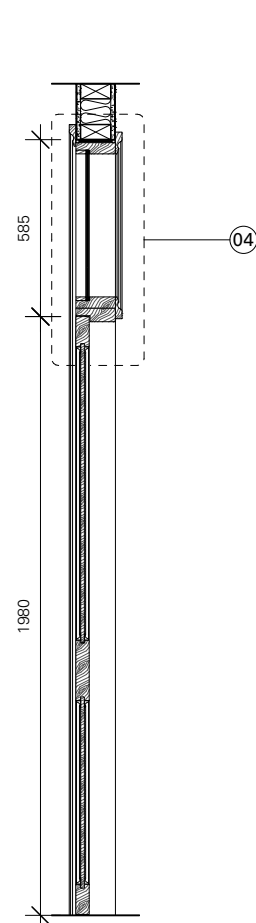
02 Section as proposed - 1:25
