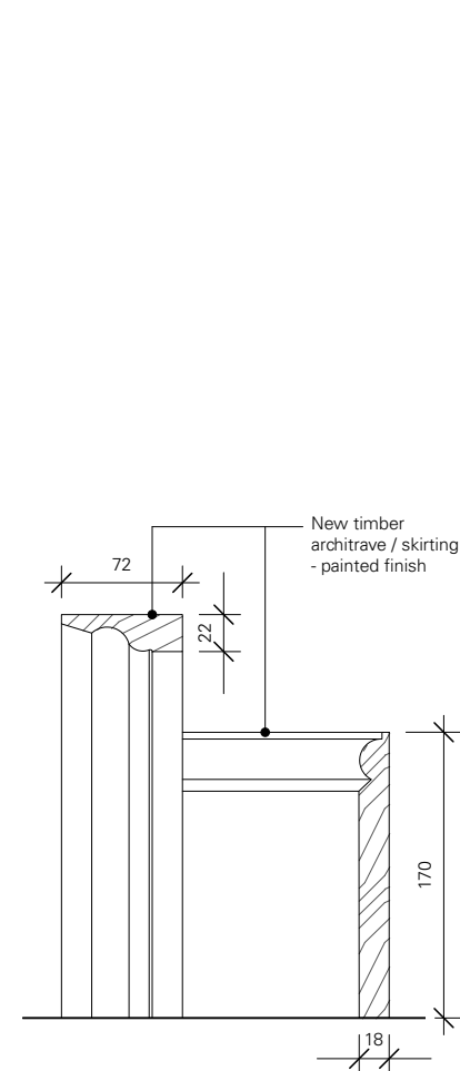
03 Skirting / Architrave - 1:5
