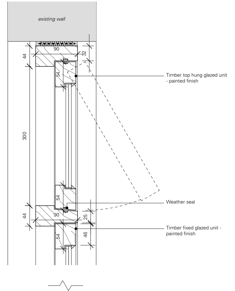
03 Head detail - 1:5
