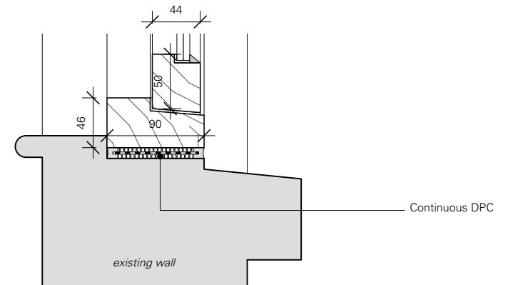
06 Cill detail - 1:5
