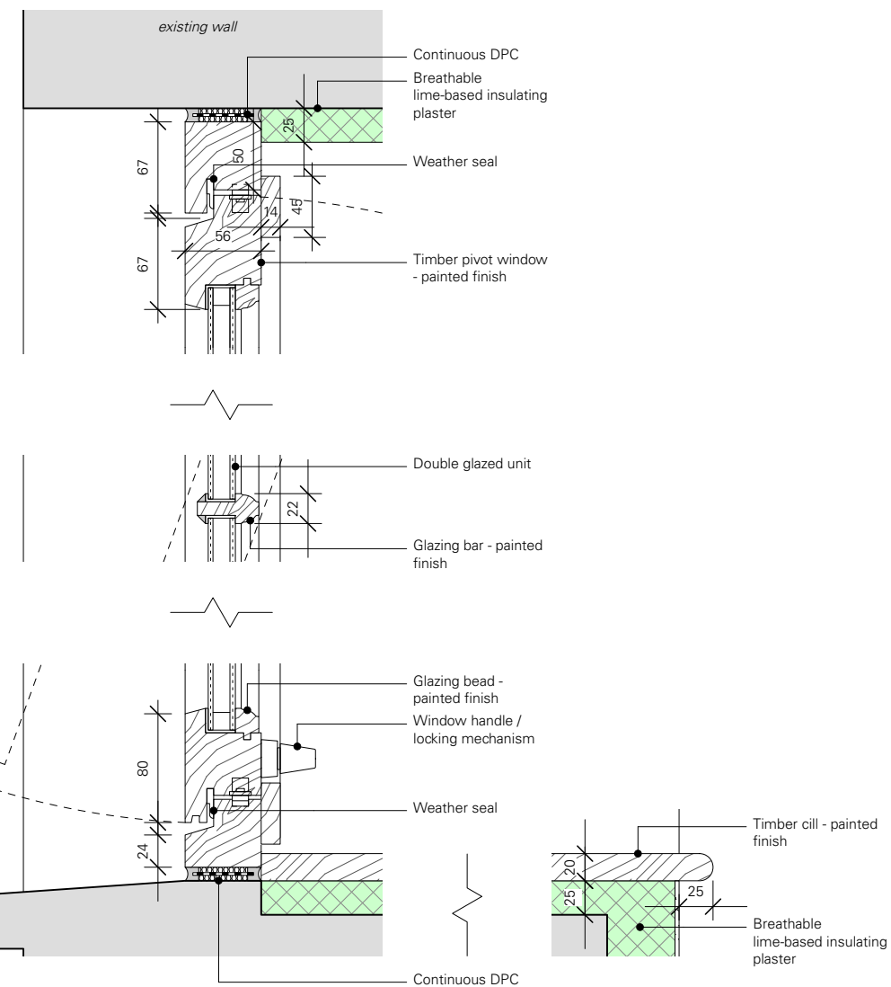
03 Section detail - 1:5
