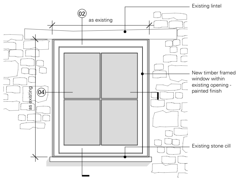
01 Elevation as proposed - 1:25
