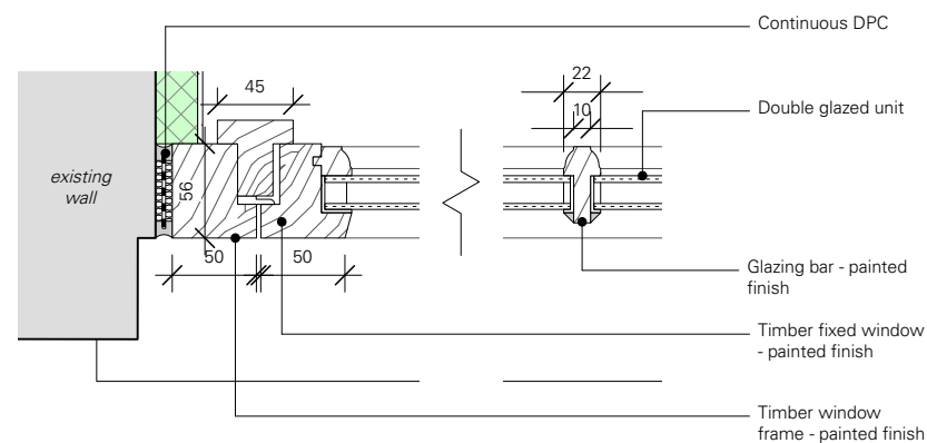
05 Plan detail - 1:5
