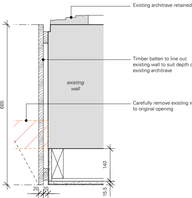
06 Plan detail - 1:10
