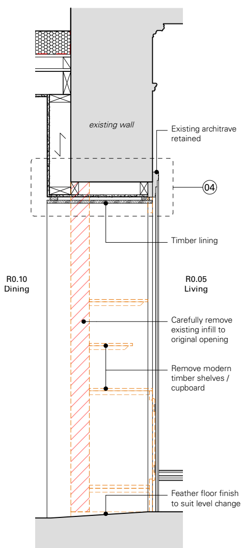
02 Section as Proposed - 1:25
