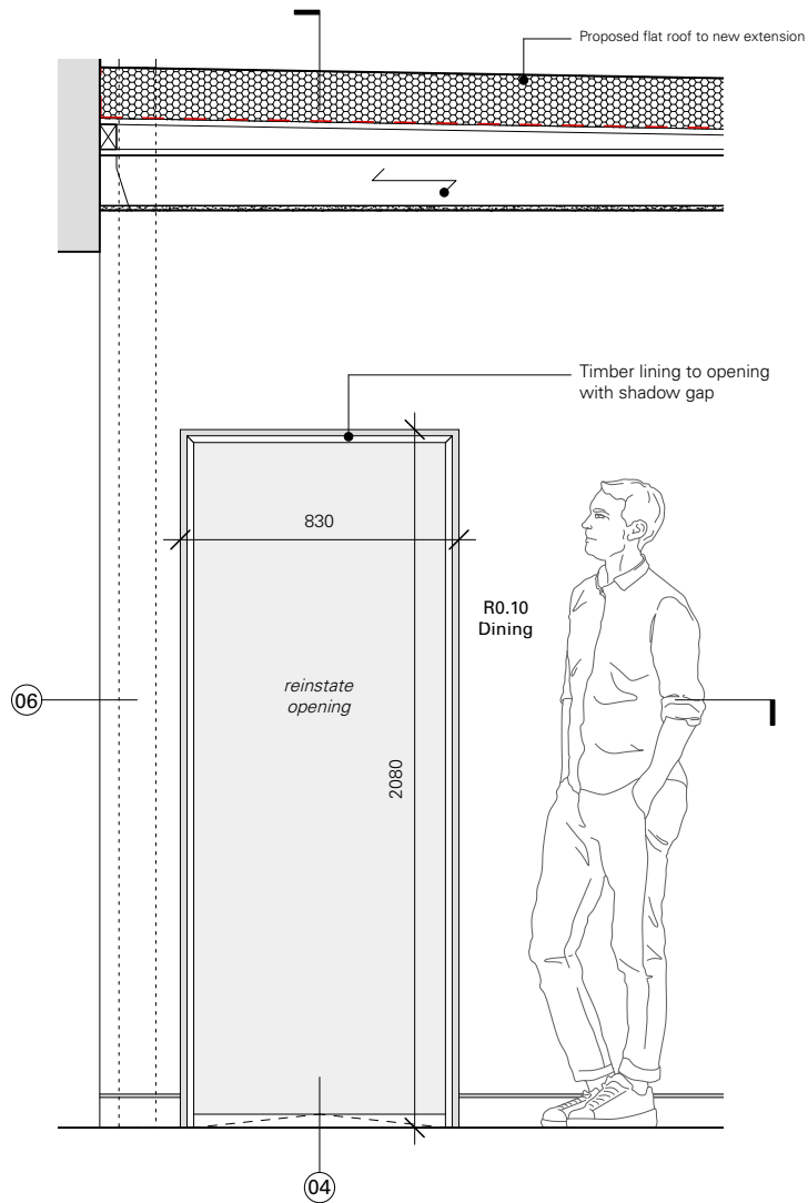
01 Elevation as Proposed (R0.10 side) - 1:25
