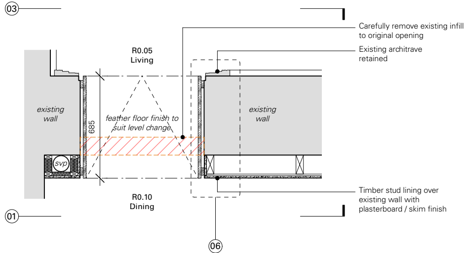
05 Plan as Proposed - 1:25
