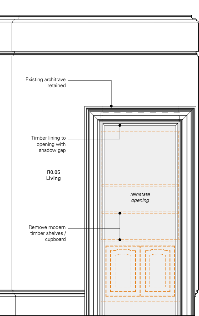
03 Elevation as Proposed (R0.05 side) - 1:25
