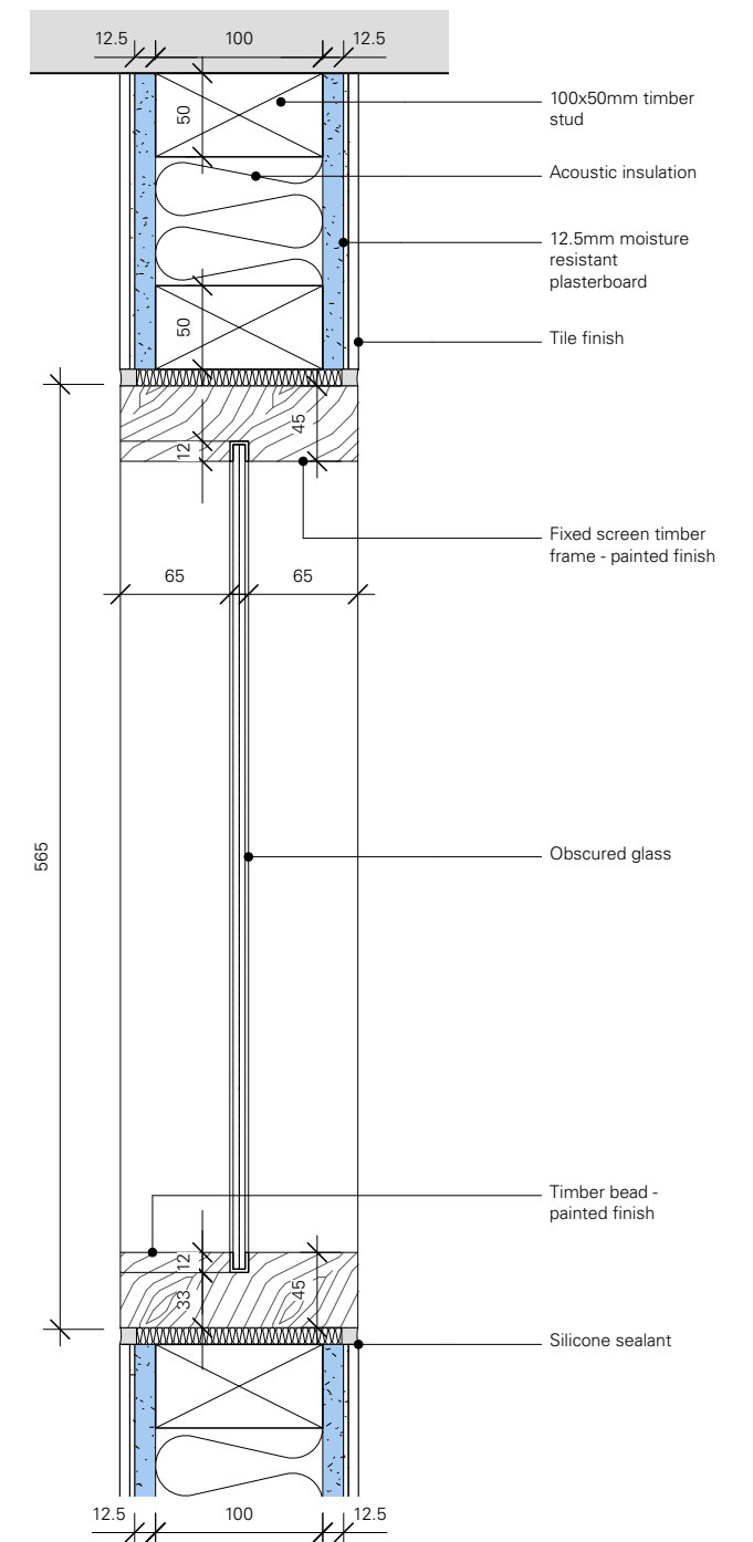
03 Section detail - 1:5
