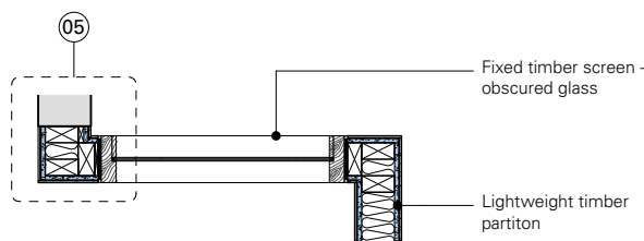
04 Fixed screen plan - 1:25
