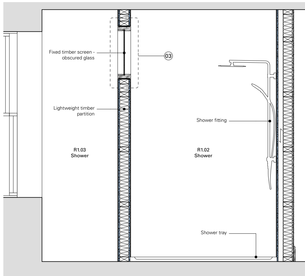
02 Section as proposed - 1:25
