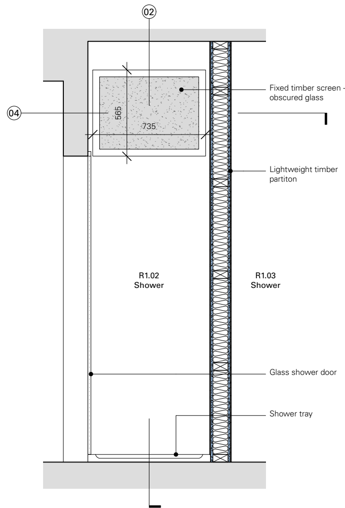
01 Elevation as proposed - 1:25
