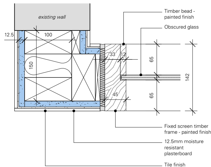
05 Plan detail - 1:5
