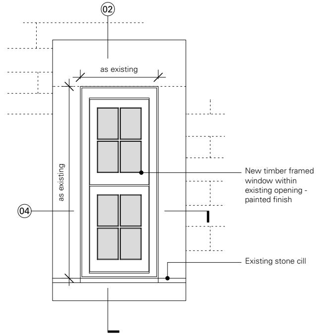
01 W11.1 + W11.2 Elevation as proposed - 1:25
