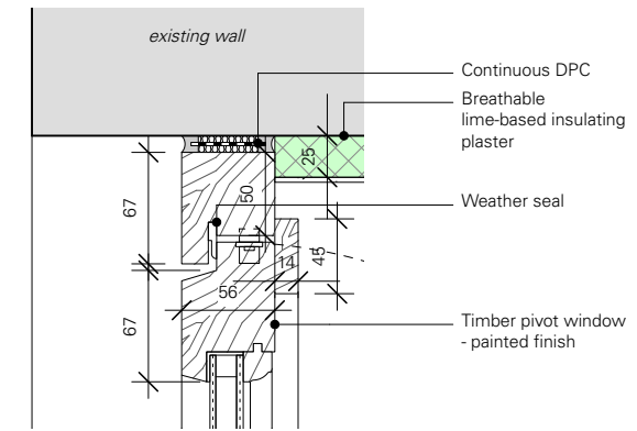
03 Section detail - 1:5
