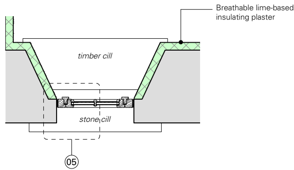
04 Plan as proposed- 1:25
