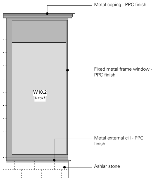
01 North elevation as proposed - 1:50
