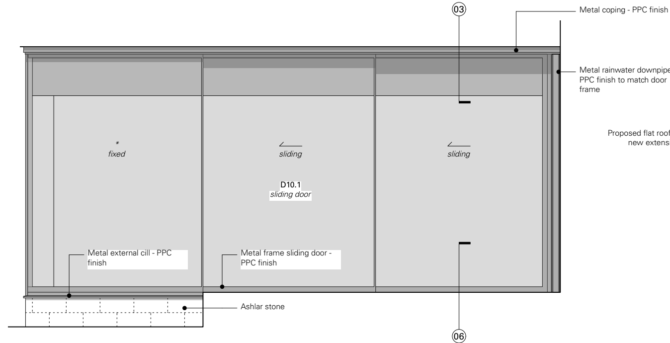
02 West elevation as proposed - 1:50
