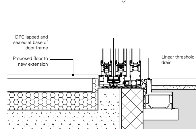
06 Cill detail - 1:10
