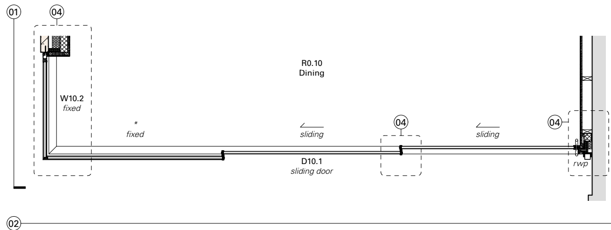
05 Plan as proposed - 1:50
