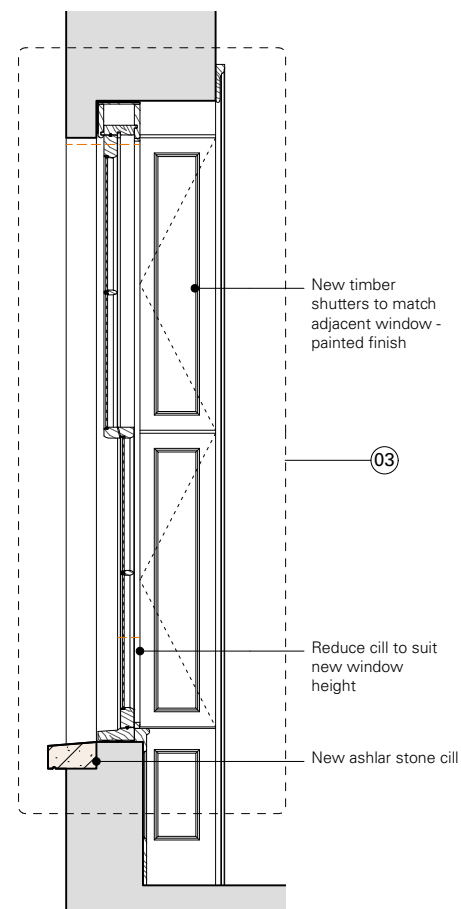
02 Section as proposed - 1:25
