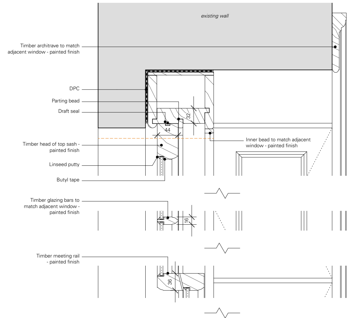
03 Section detail - 1:5
