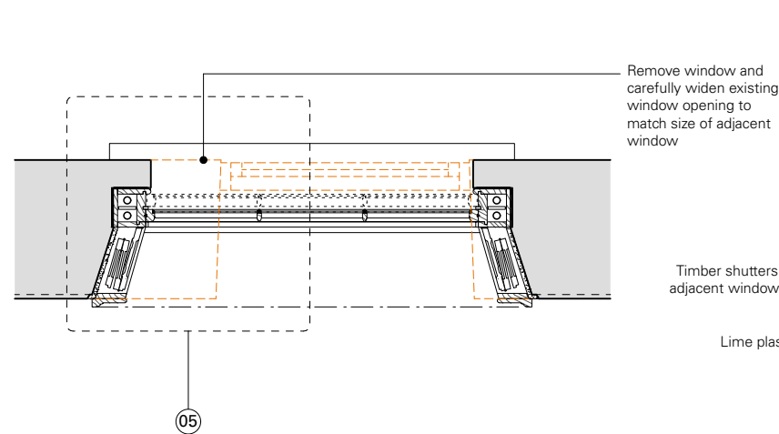
04 Plan as proposed - 1:25
