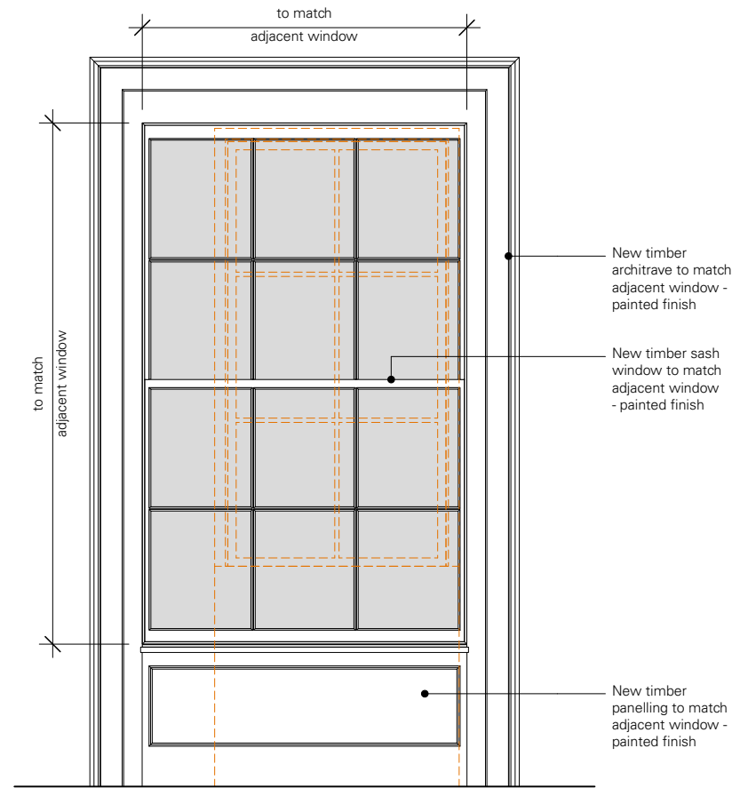
01 Elevation as proposed - 1:25
