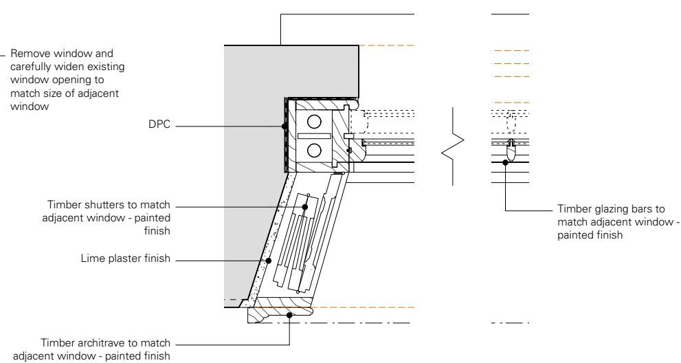
05 Plan Detail - 1:10
