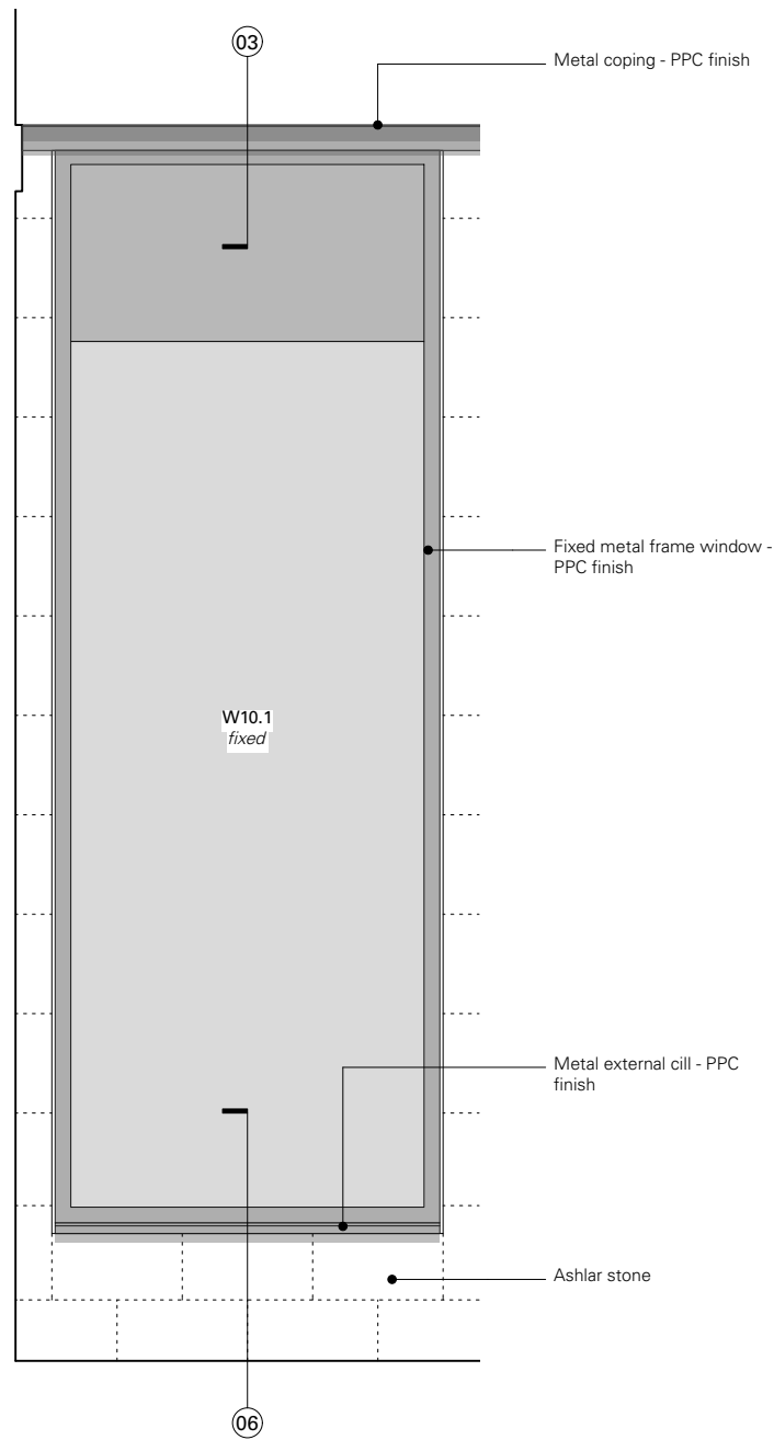
01 Elevation as proposed - 1:25
