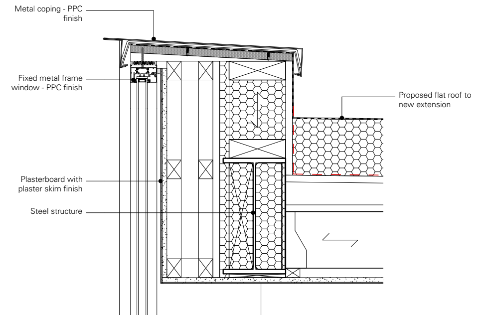
03 Head detail - 1:10
