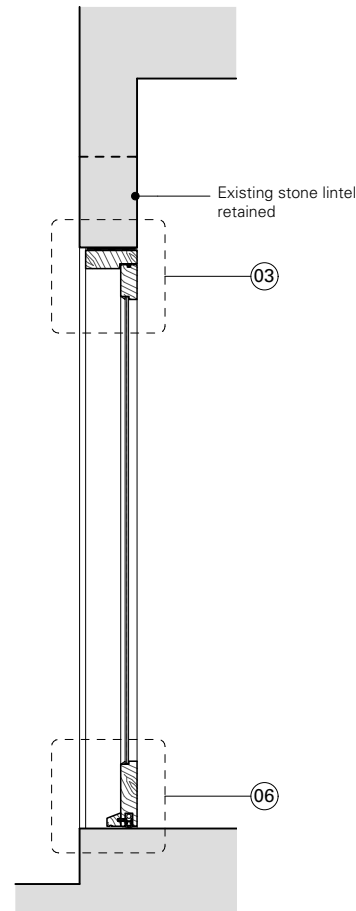
02 Section as proposed - 1:25
