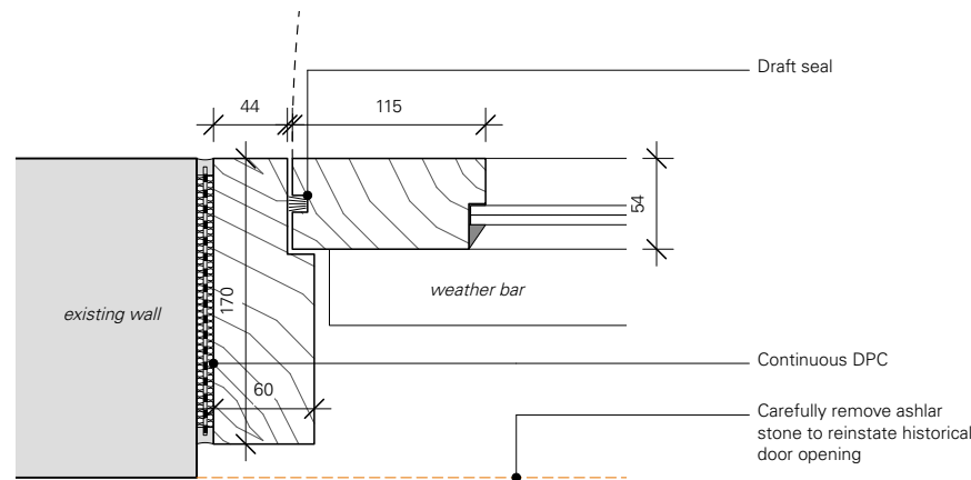
05 Plan detail - 1:5
