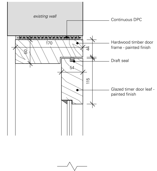
03 Head detail - 1:5
