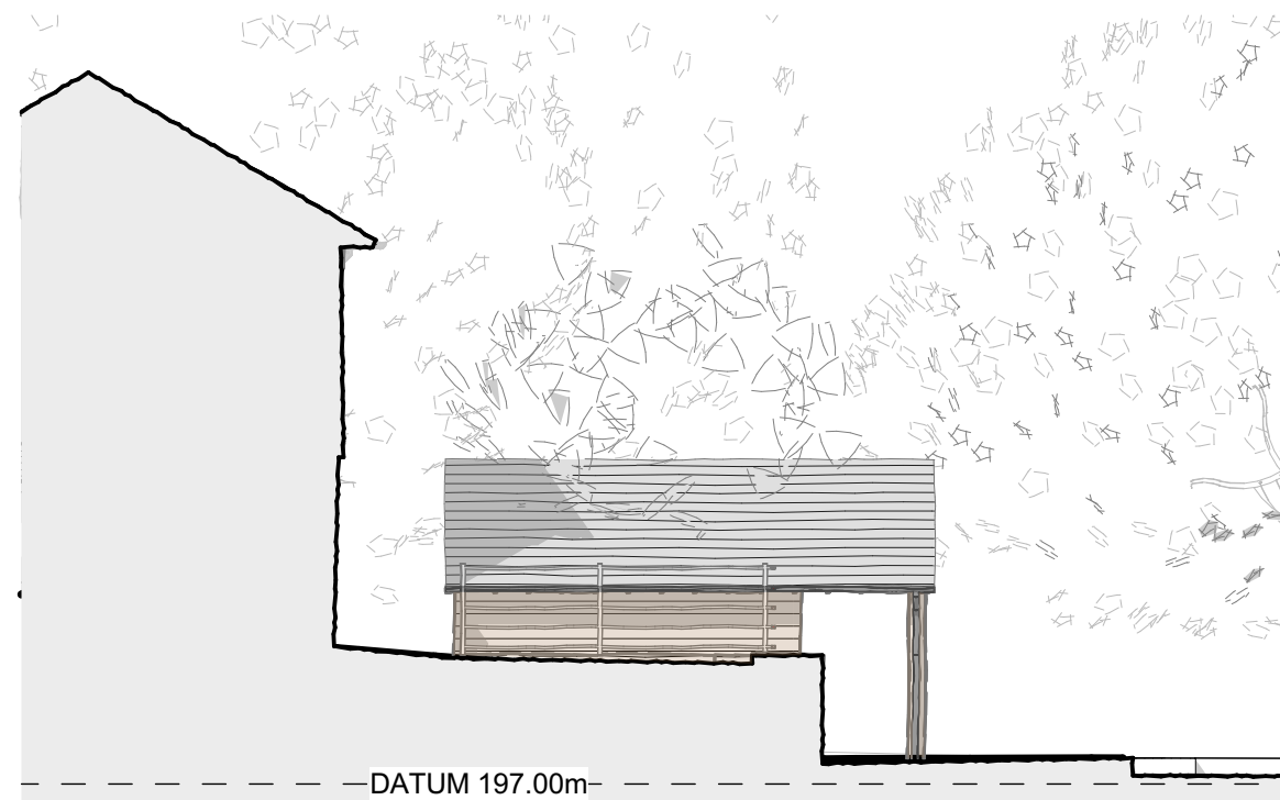
POOL HOUSE WEST ELEVATION
