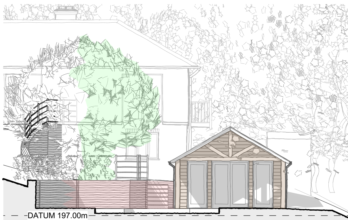
POOL HOUSE SOUTH ELEVATION
