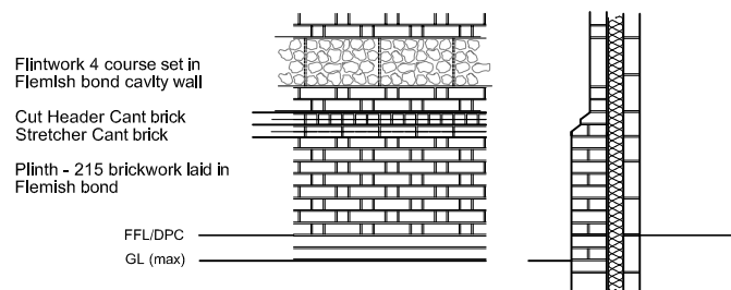
WALL DETAIL
