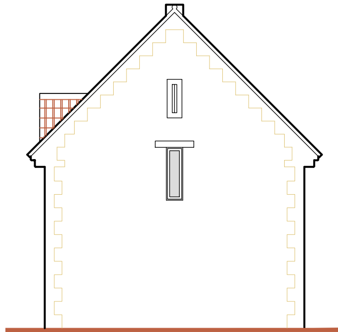
North Elevation
