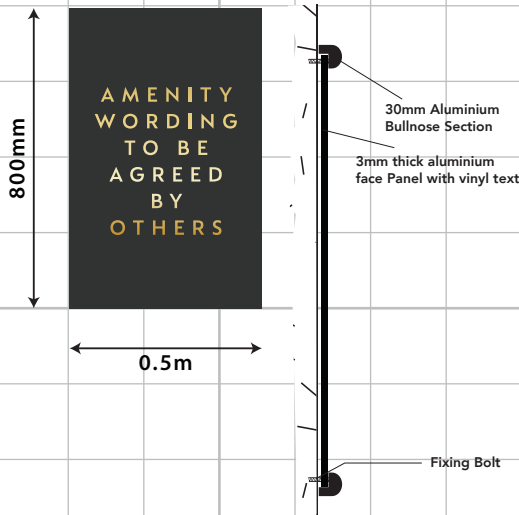
E ONE X AMENITY BOARD. SIZE. 0.5m x 800mm. H.A.G. 0.85m.
