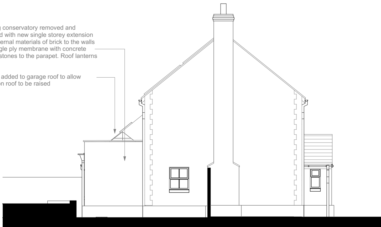
E-02 East Elevation 1:100
