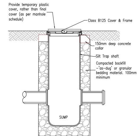
CATCHPIT/SILT TRAP
