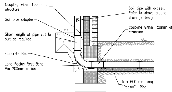
SOIL & VENT PIPE/STUB STACK/WC CONNECTION
