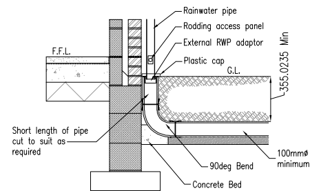
EXTERNAL RAINWATER PIPE CONNECTION
