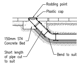
RODDING POINT/EYE
