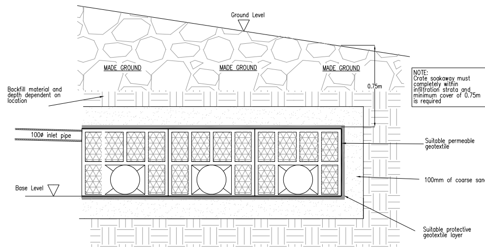
AQUACELL SOAKAWAY - PRIME UNITS
