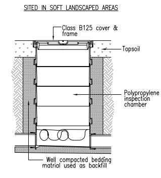
POLYPROPYLENE INSPECTION CHAMBER INSTALLATION
