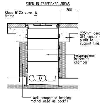
POLYPROPYLENE INSPECTION CHAMBER INSTALLATION
