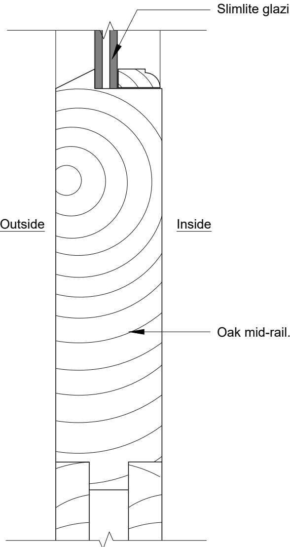
D2- Mid Rail Detail Scale 1:2
