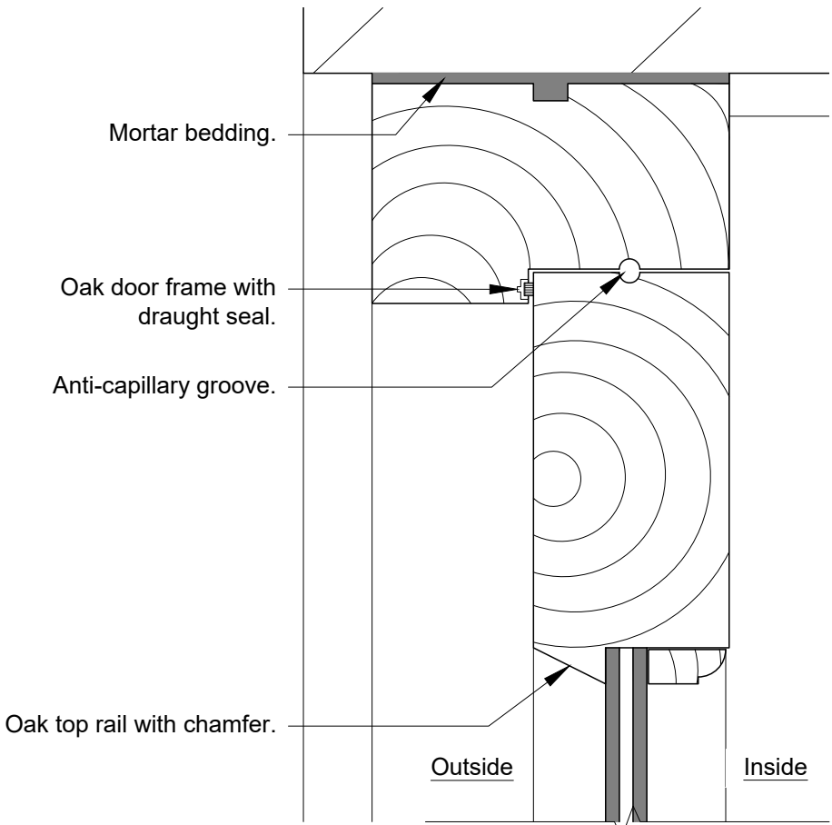
D1- Door Head & Top Rail Detail Scale 1:2
