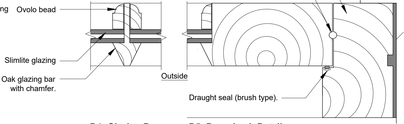
D4- Glazing Bar Detail Scale 1:2
