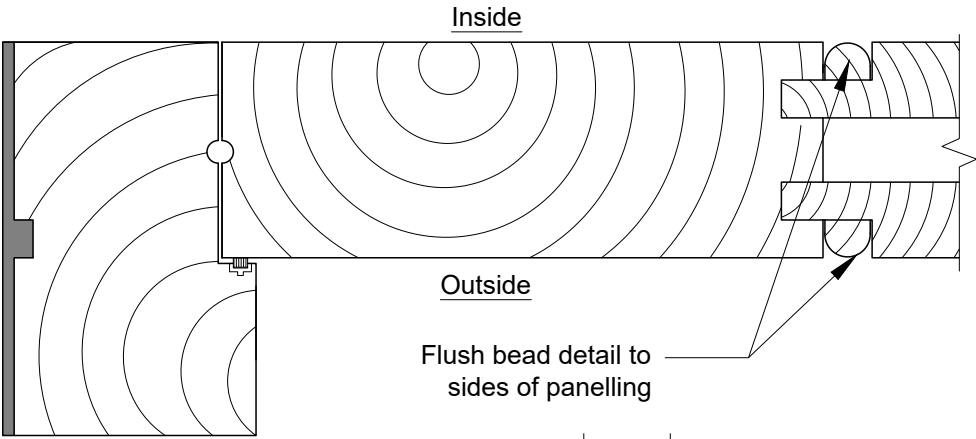
D6- Panelling Detail Scale 1:2
