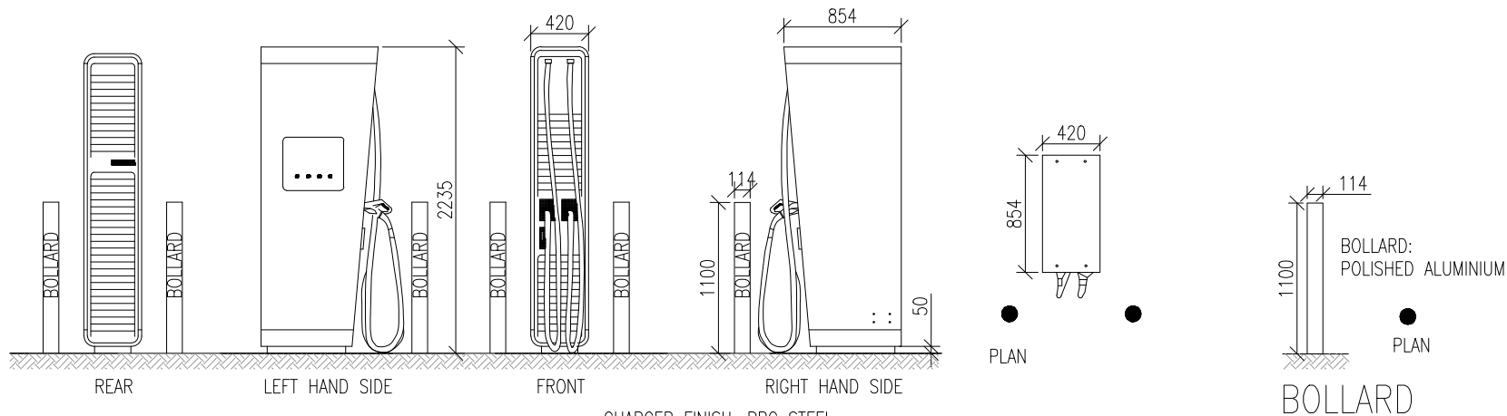
ELEVATIONS HYC_150 DC CHARGER CHARGER FINISH: PPC STEEL COLOUR: BLACK WITH POLISHED ALUMINIUM
