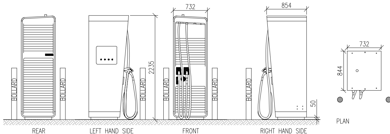
ELEVATIONS HYC_300 DC CHARGER CHARGER FINISH: PPC STEEL COLOUR: BLACK WITH POLISHED ALUMINIUM
