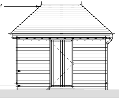
FRONT (SOUTH EAST) ELEVATION
