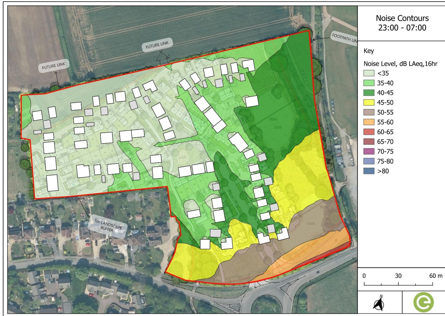
Figure B4: Night-time Noise Contour
