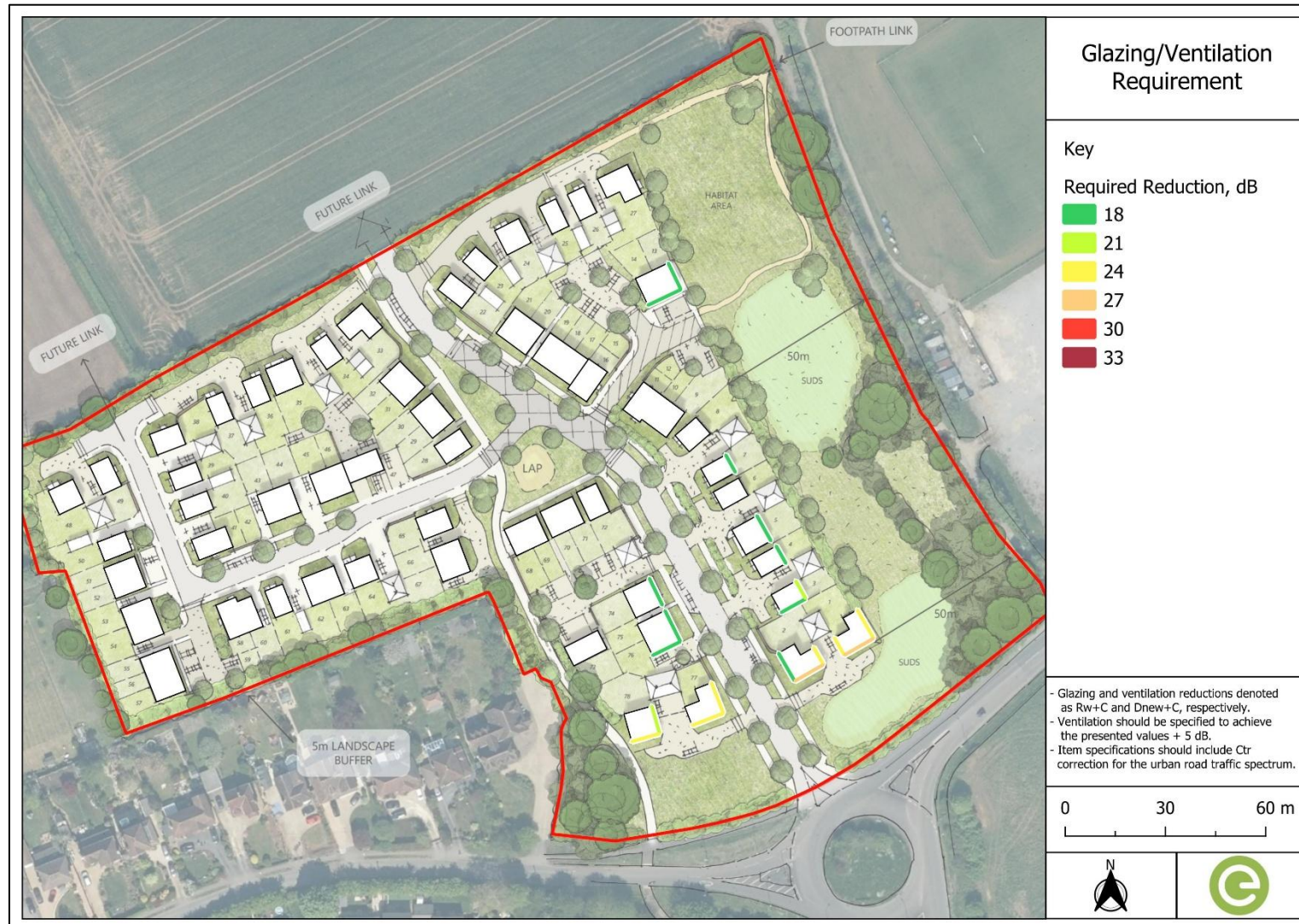
Figure B5: Calculated Façade Mitigation Requirements
