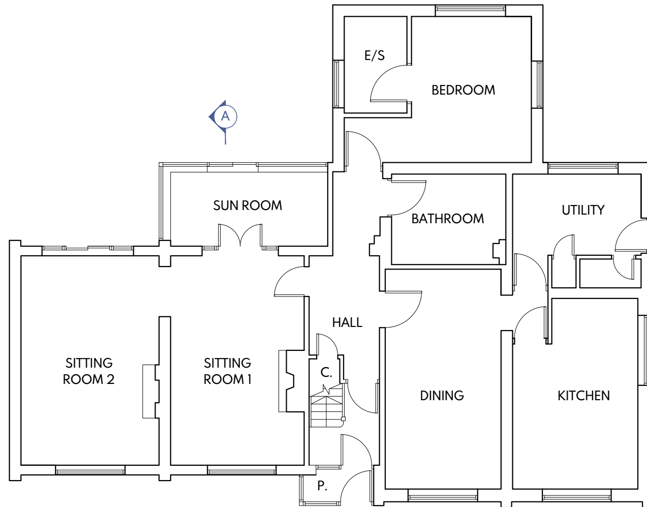
GROUND FLOOR 1:100
