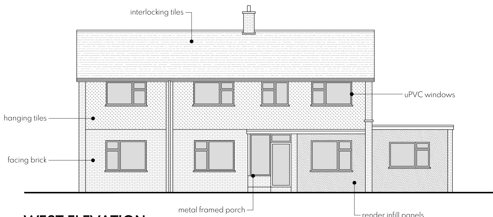
WEST ELEVATION 1:100
