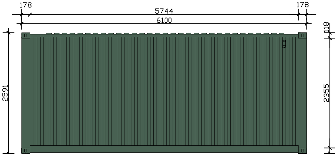
Side view
