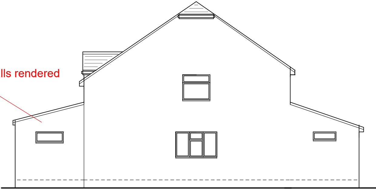
right side (southeast) elevation
