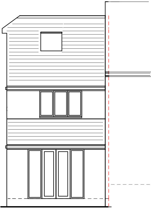
rear (northeast) elevation
