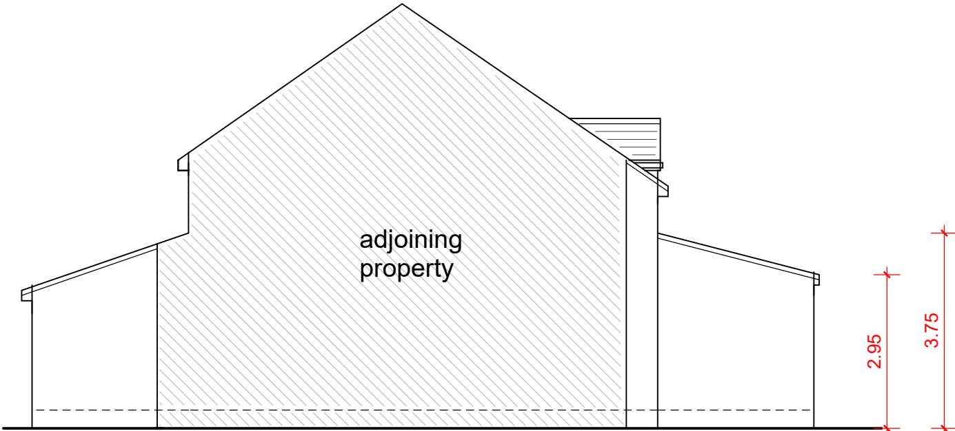
left side (northwest) elevation
