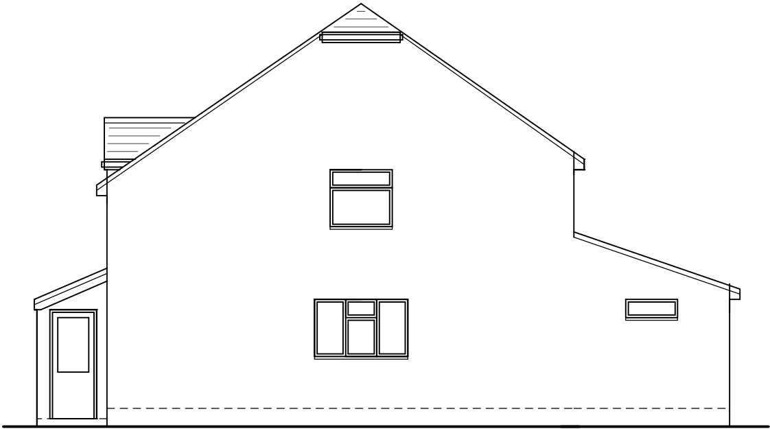
right side (southeast) elevation
