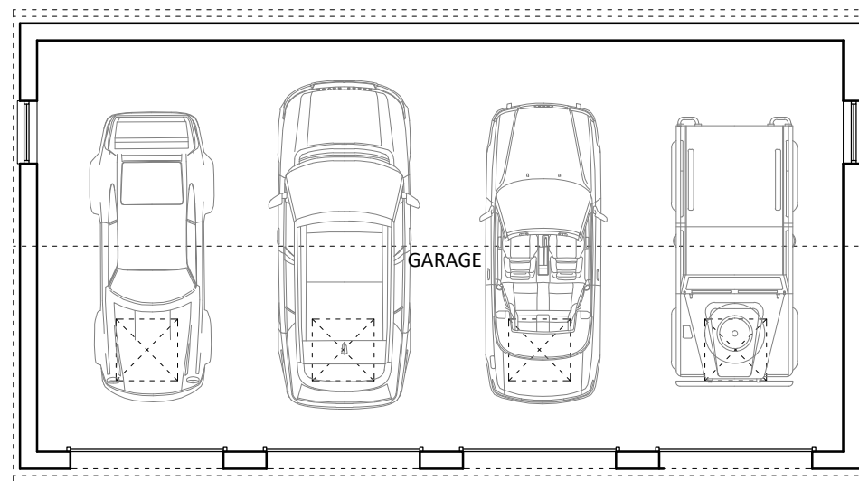
PLAN - scale 1:100
