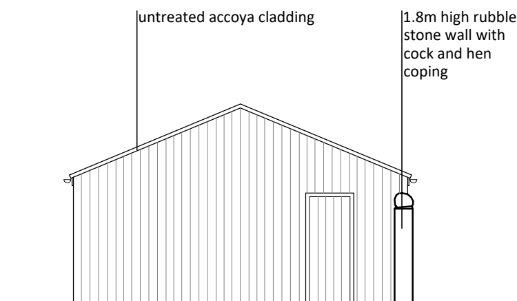
SIDE (N) ELEVATION - scale 1:100
