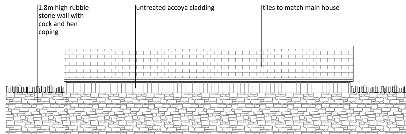
STREET (W) ELEVATION - scale 1:100
