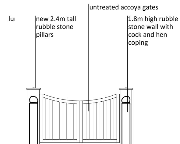
ENTRY GATES - scale 1:100
