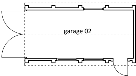
GROUND FLOOR PLAN - scale 1:100
