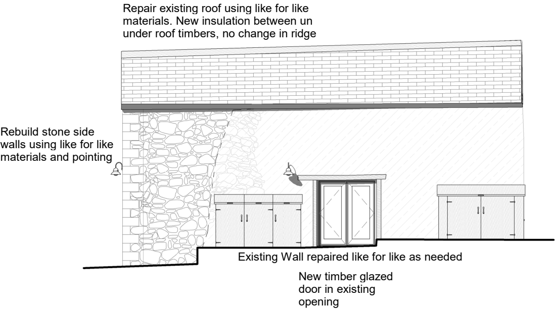
Dairy Barn Proposed Rear (North) 1 : 100
