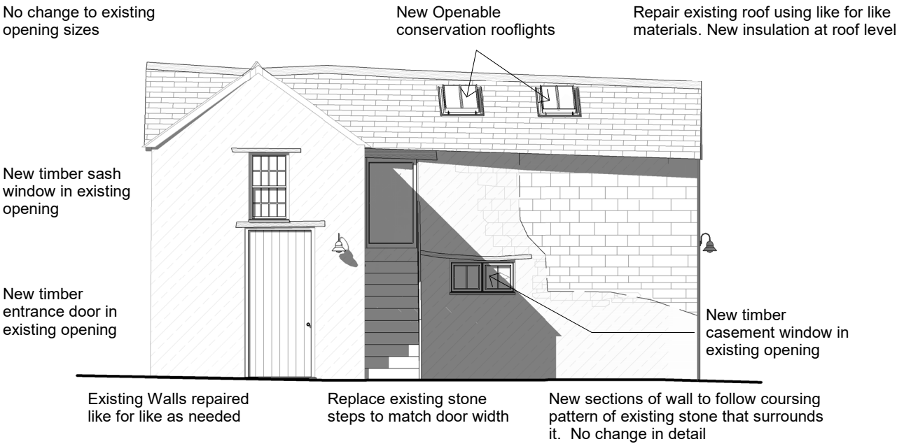
Dairy Barn Proposed South 1 : 100
