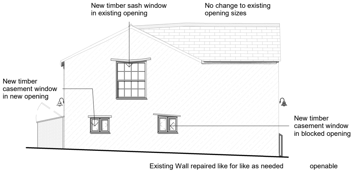
Dairy Barn Proposed West 1 : 100
