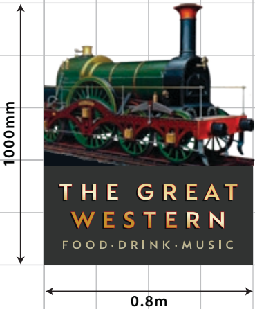
F ONE X NEW DOUBLE SIDED PANEL TO EXISTING POST SIGN. ILLUMINATED BY LINOLITES. (NOT SHOWN) SIZE. 0.8m x 1000mm. H.A.G. 3.5m.
