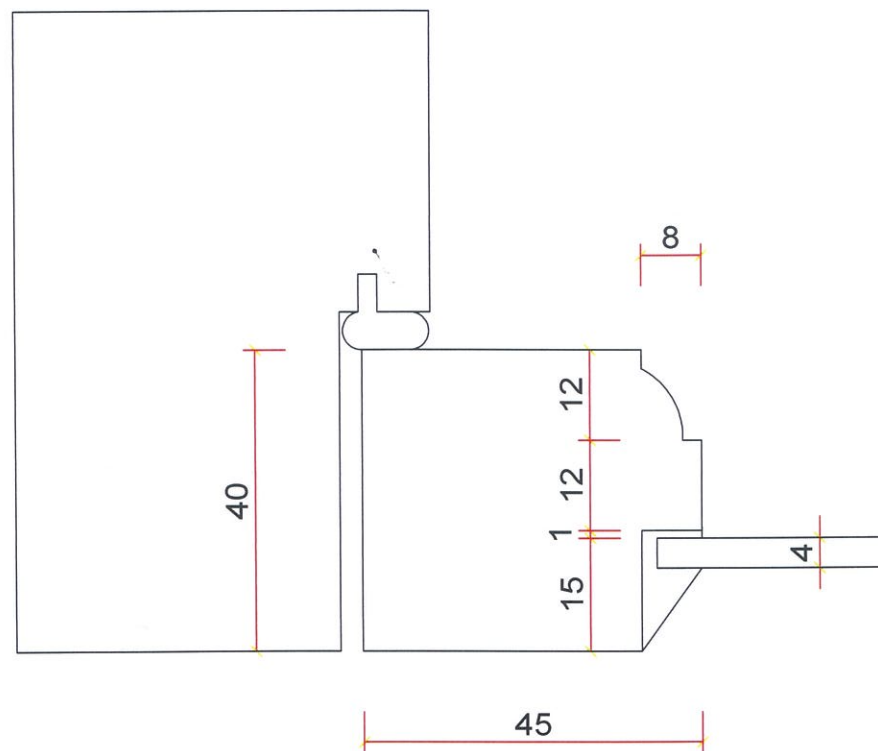
Frame & casement section for W4 W5 & W6 No 4A Northgate St
