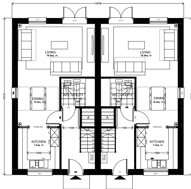
GROUND FLOOR PLAN 1:50
