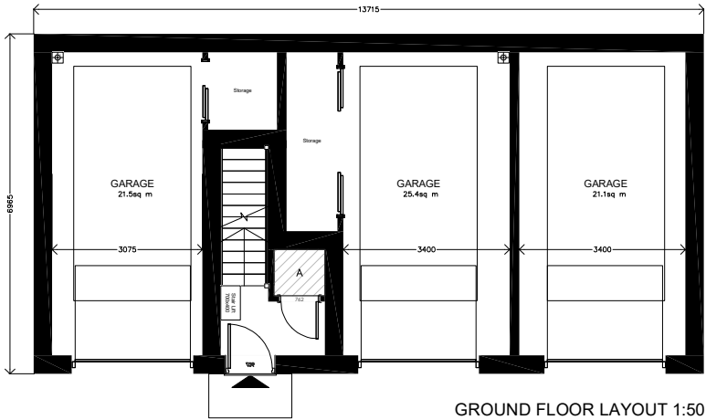
GROUND FLOOR LAYOUT 1:50
