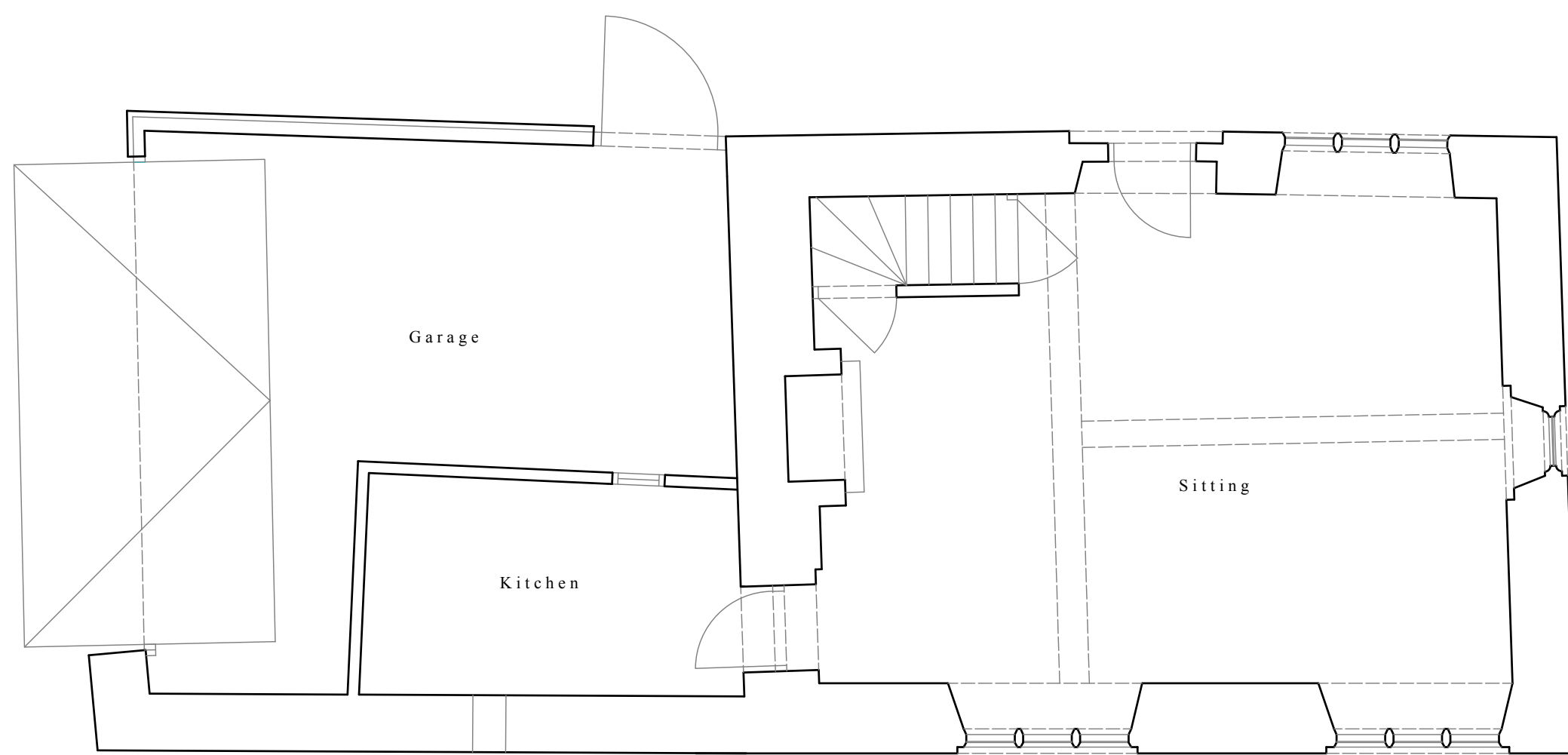
GROUND FLOOR
