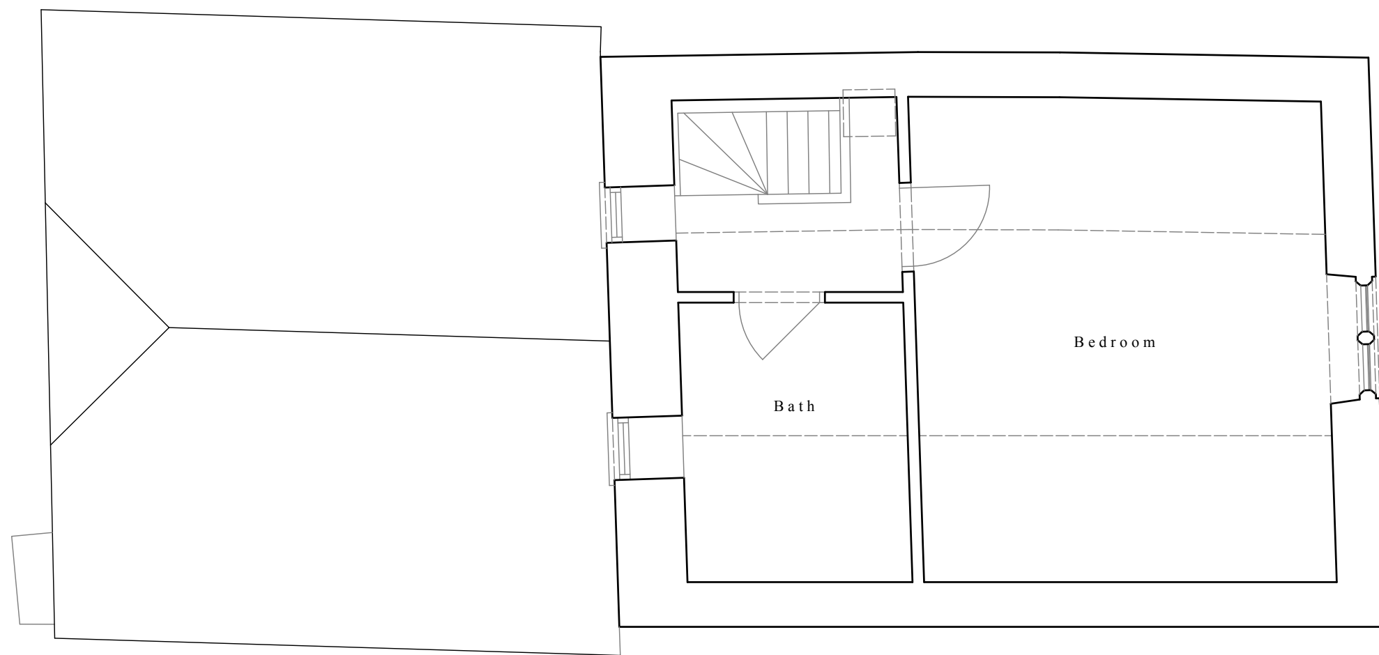
FIRST FLOOR
