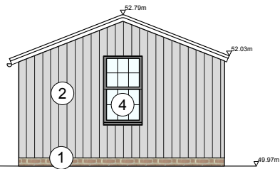
ELEVATION G GARAGE SOUTH-EAST
