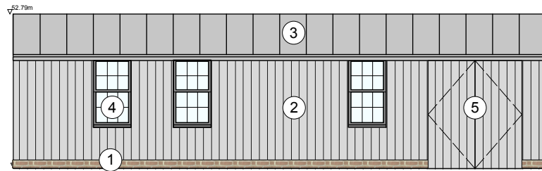
ELEVATION H GARAGE NORTH-EAST
