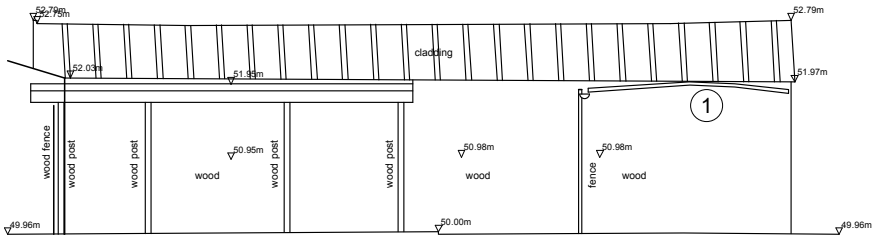
ELEVATION F GARAGE SOUTH-WEST
