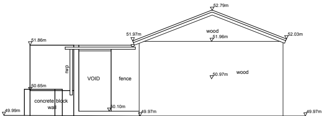
ELEVATION G GARAGE SOUTH-EAST
