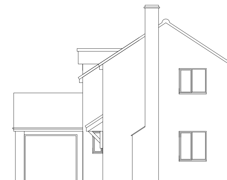
Proposed North East Elevation 1:100
