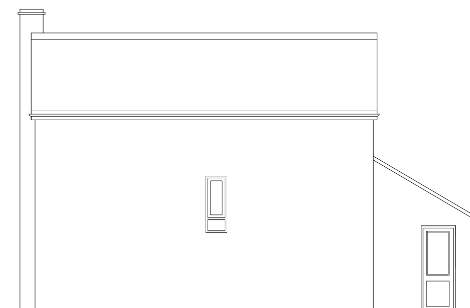
Existing North West Elevation 1:100
