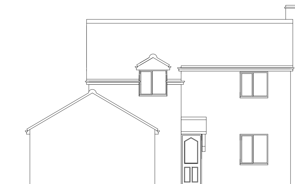
Proposed South East Elevation 1:100
